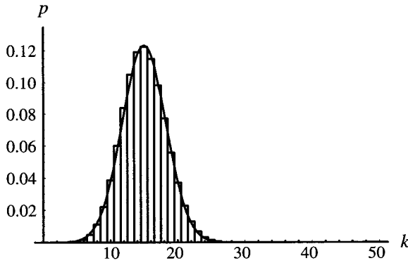
Figure 2 An approximation of binomial probabilities
