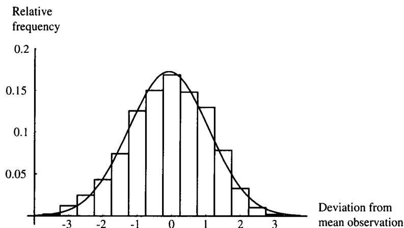
Figure 7 Normally distributed measurements
