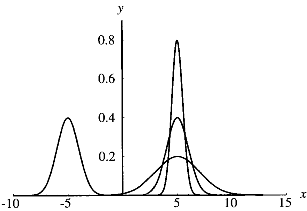
Figure 1 Bell-shaped curves
