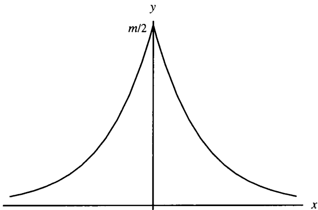
Figure 5 Laplace's first error curve
